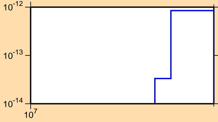
\sigma vs. E for ^{163}\text{Er} (mt 45)
