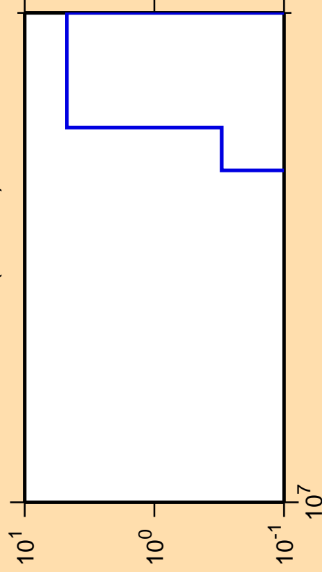
\Delta\sigma/\sigma vs. E for ^{163}\text{Er}(\text{mt117})
