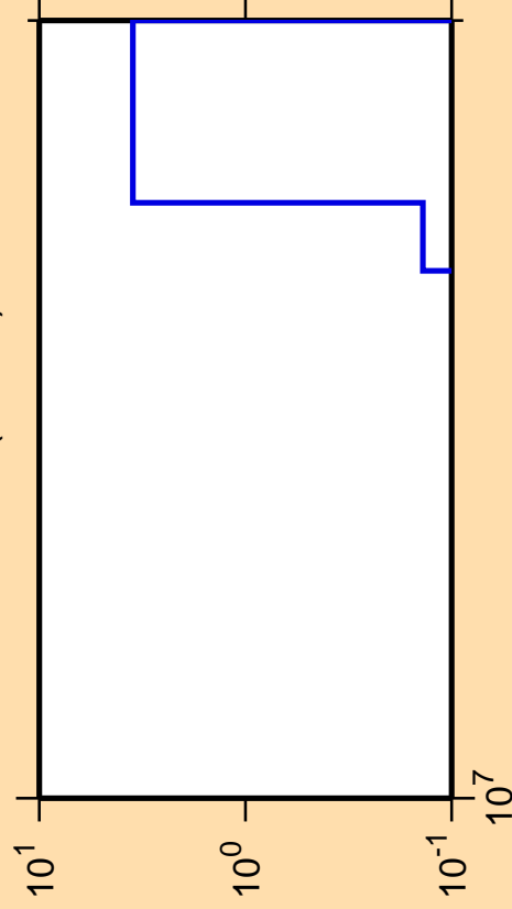
\Delta\sigma/\sigma vs. E for ^{163}\text{Er} (mt 45)
