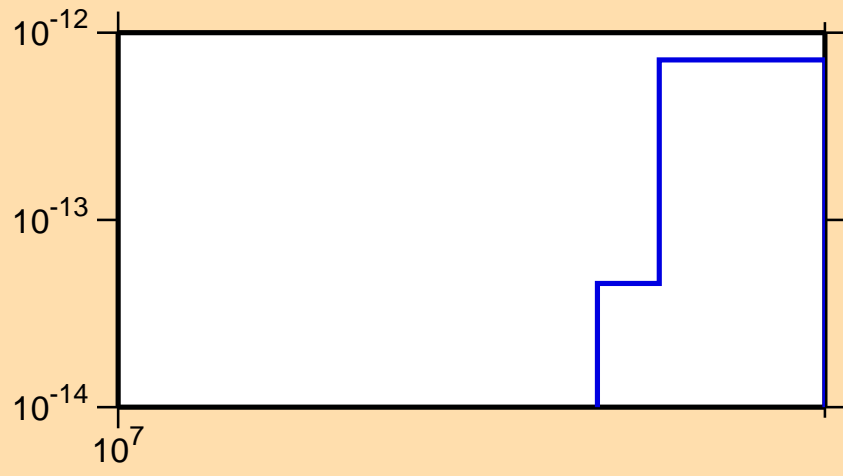
\sigma vs. E for ^{163}\text{Er}(\text{mt117})
