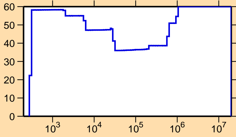
\Delta\sigma/\sigma vs. E for ^{163}\text{Er}(n,\gamma)
