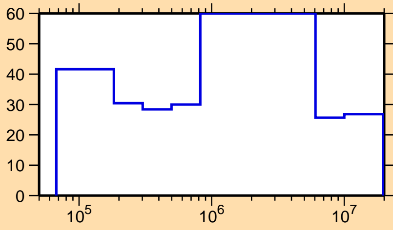
\Delta\sigma/\sigma vs. E for ^{163}\text{Er}(n,n_1)
