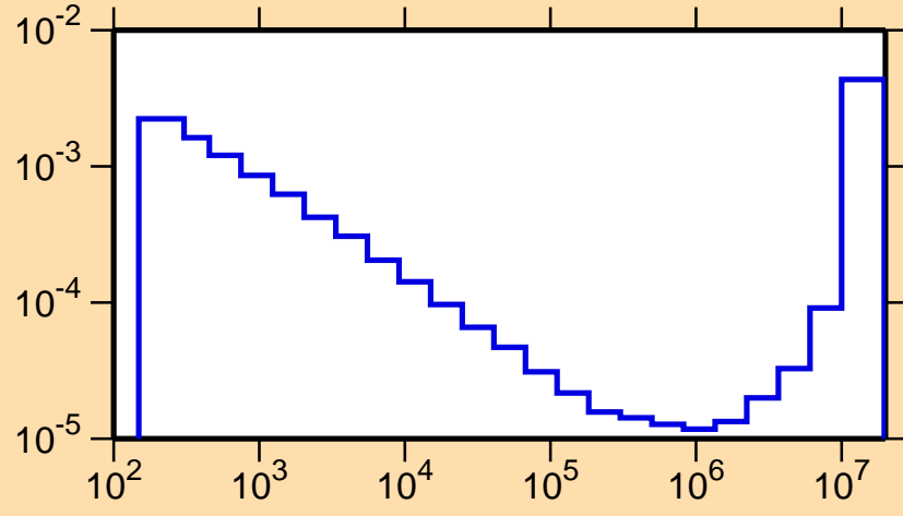
\sigma vs. E for ^{163}\text{Er}(n,\alpha)
