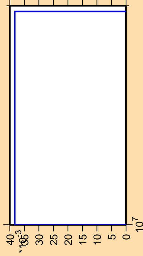
\Delta\sigma/\sigma vs. E for ^{163}\text{Er} (mt 45)
