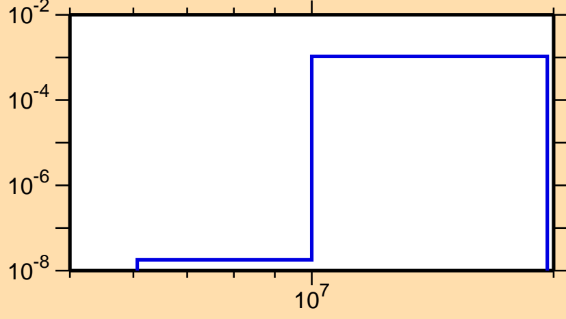
\sigma vs. E for ^{163}\text{Er}(n,d)
