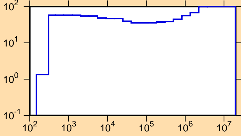
\Delta\sigma/\sigma vs. E for ^{163}\text{Er}(n,\gamma)
