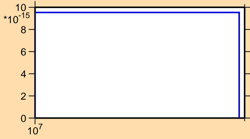
\sigma vs. E for ^{163}\text{Er} (mt 45)
