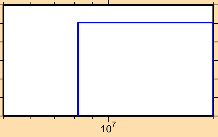
\sigma vs. E for ^{163}\text{Er}(n,2n\alpha)
