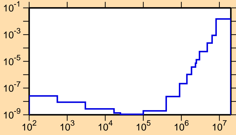
\sigma vs. E for ^{163}\text{Er}(n,p)
