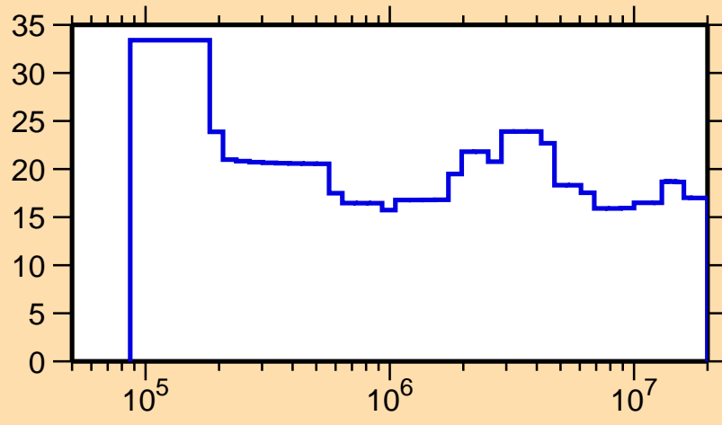
\Delta\sigma/\sigma vs. E for ^{164}\text{Er}(n,n_1)
