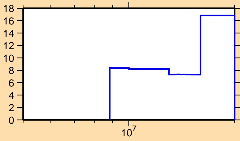
\Delta\sigma/\sigma vs. E for ^{164}\text{Er}(n,2n)
