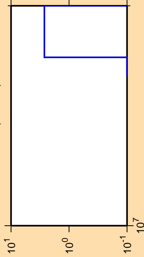
\Delta\sigma/\sigma vs. E for ^{164}\text{Er}(\text{mt117})
