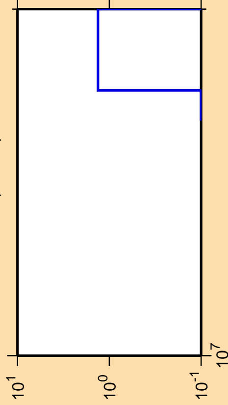
\Delta\sigma/\sigma vs. E for ^{164}\text{Er} (mt 45)
