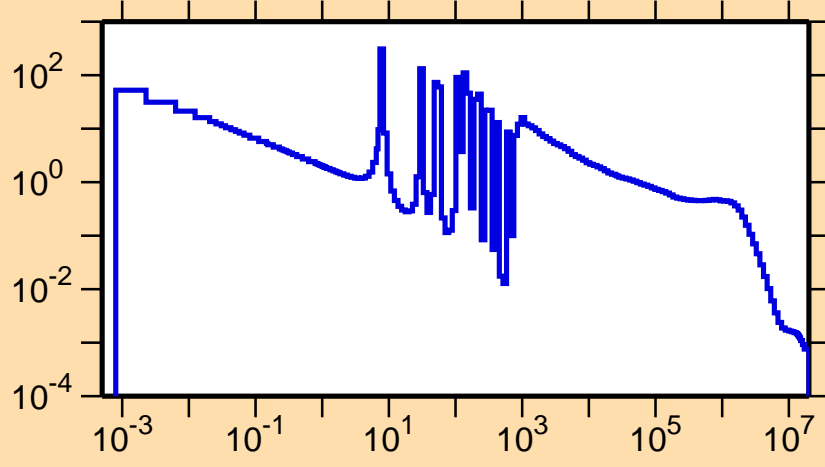
\sigma vs. E for ^{164}\text{Er}(n,\gamma)
