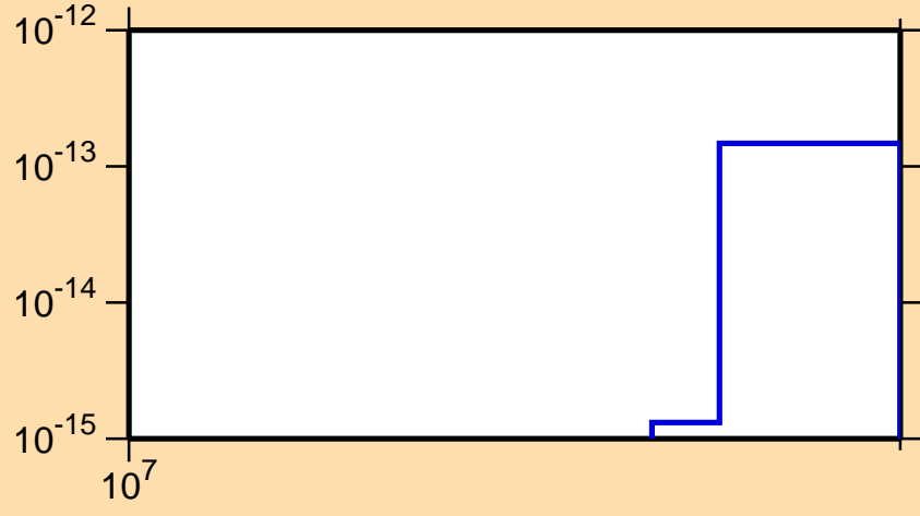
\sigma vs. E for ^{164}\text{Er} (mt 45)
