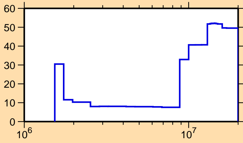
\Delta\sigma/\sigma vs. E for ^{164}\text{Er}(n,n\text{cont.})
