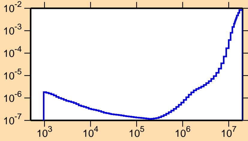
\sigma vs. E for ^{164}\text{Er}(n,\alpha)
