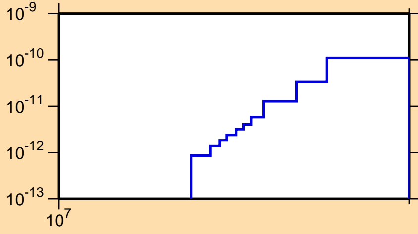
\sigma vs. E for ^{164}\text{Er}(n,p\alpha)
