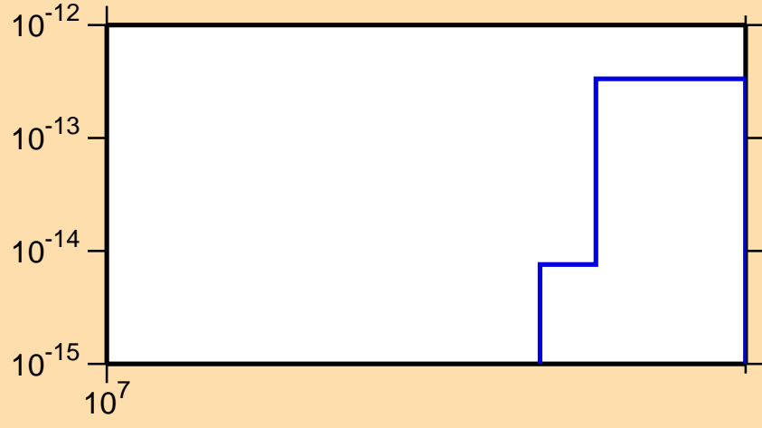
\sigma vs. E for ^{164}\text{Er}(\text{mt117})
