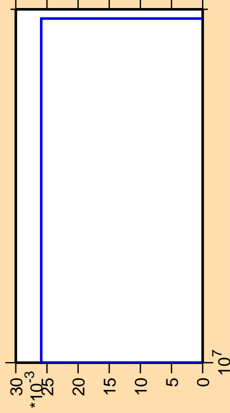
\Delta\sigma/\sigma vs. E for ^{164}\text{Er}(\text{mt117})
