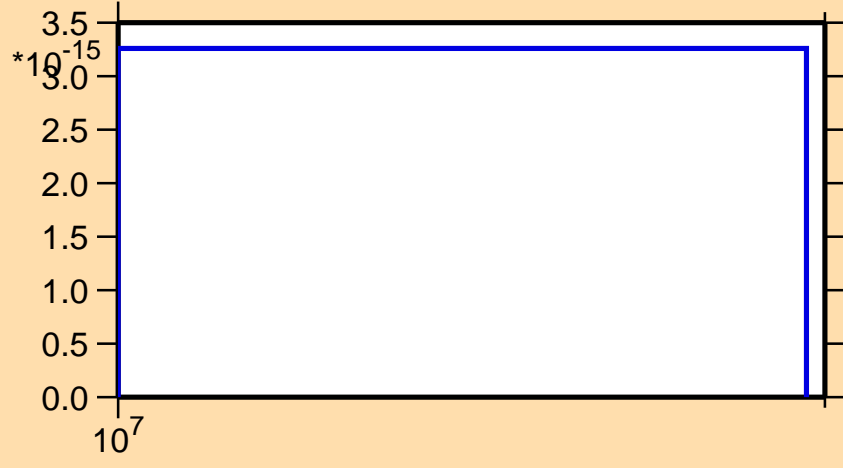
\sigma vs. E for ^{164}\text{Er}(\text{mt117})
