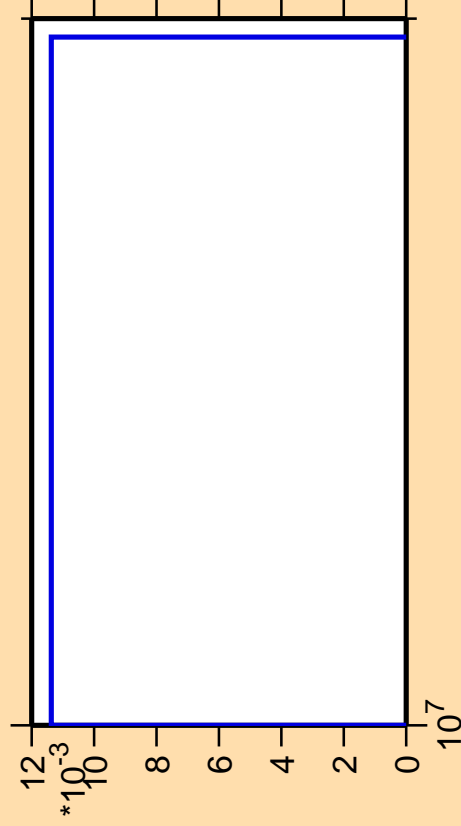
\Delta\sigma/\sigma vs. E for ^{164}\text{Er} (mt 45)
