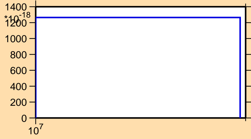
\sigma vs. E for ^{164}\text{Er} (mt 45)
