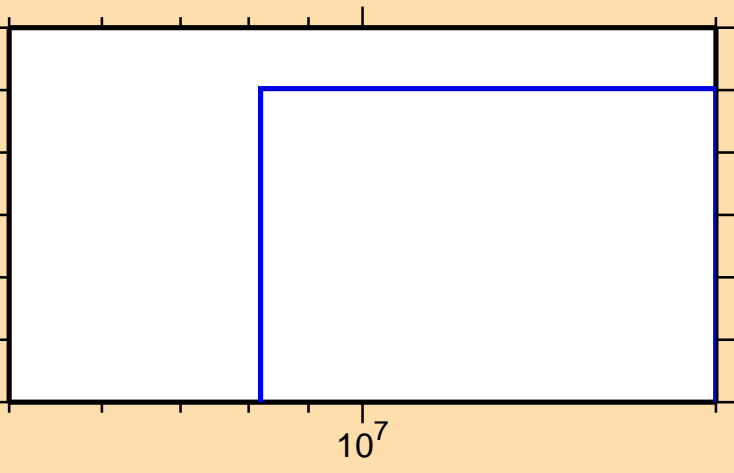
\sigma vs. E for ^{164}\text{Er}(n,p\alpha)
