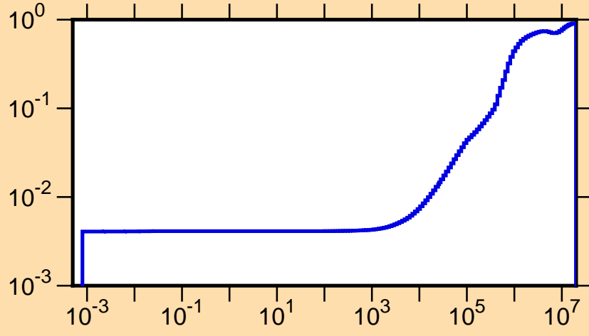
\mu vs. E for ^{165}\text{Er}(\text{mt251})
