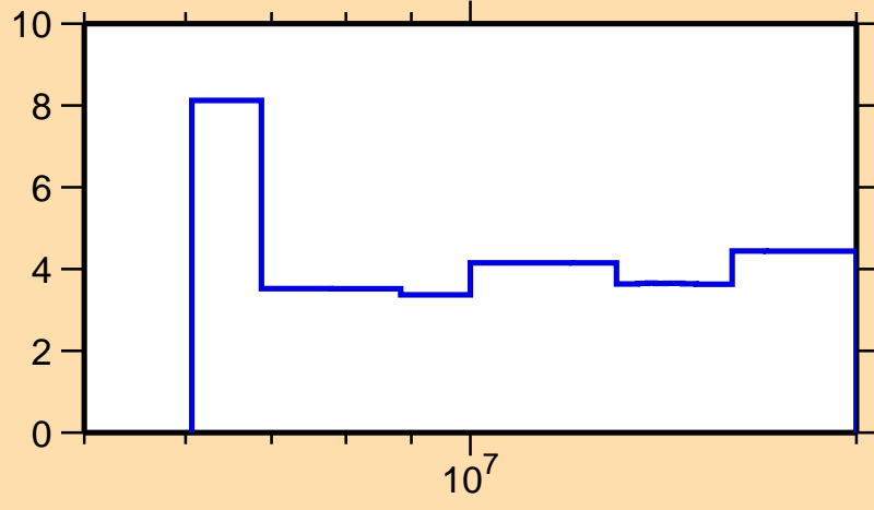
\Delta\sigma/\sigma vs. E for ^{165}\text{Er}(n,\text{tot.})
