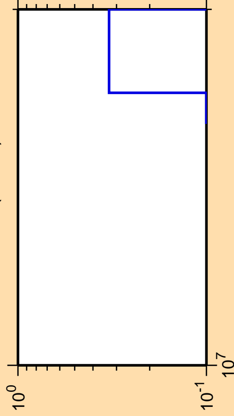
\Delta\sigma/\sigma vs. E for ^{165}\text{Er} (mt 34)
