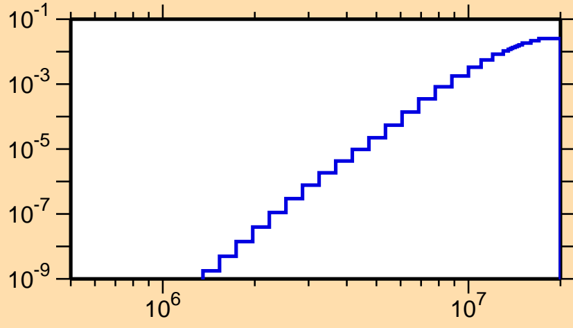
\sigma vs. E for ^{165}\text{Er}(n,p)
