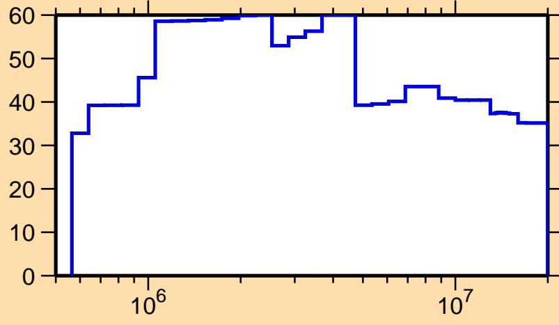
\Delta\sigma/\sigma vs. E for ^{165}\text{Er}(n,n_1)
