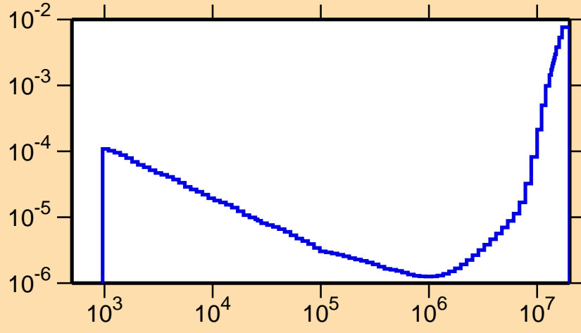
\sigma vs. E for ^{165}\text{Er}(n,\alpha)
