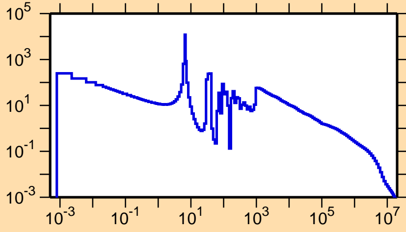
\sigma vs. E for ^{165}\text{Er}(n,\gamma)
