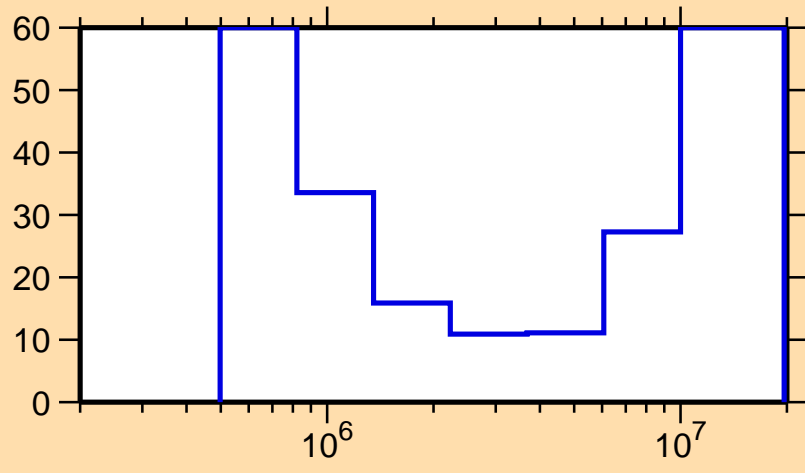
\Delta\sigma/\sigma vs. E for ^{165}\text{Er}(n,n\text{cont.})
