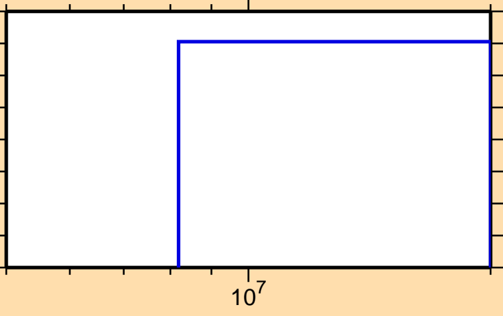
\sigma vs. E for ^{165}\text{Er}(n,2np)
