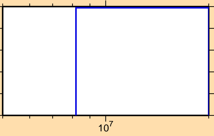
\sigma vs. E for ^{165}\text{Er}(n,2n\alpha)
