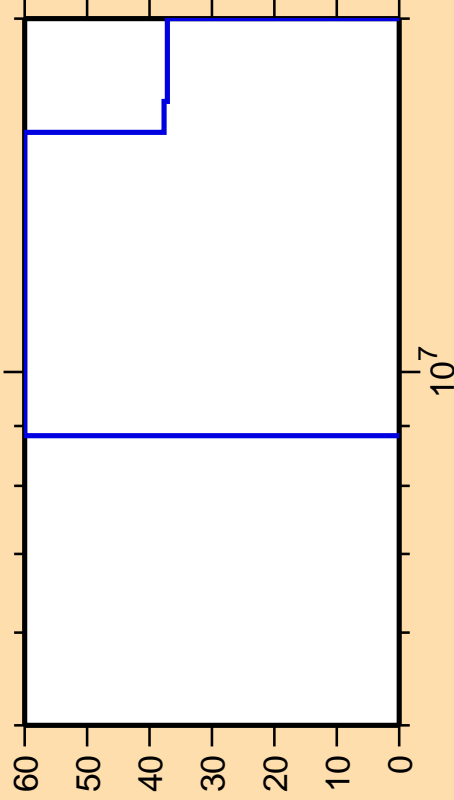
\Delta\sigma/\sigma vs. E for ^{166}\text{Er}(n,np)
