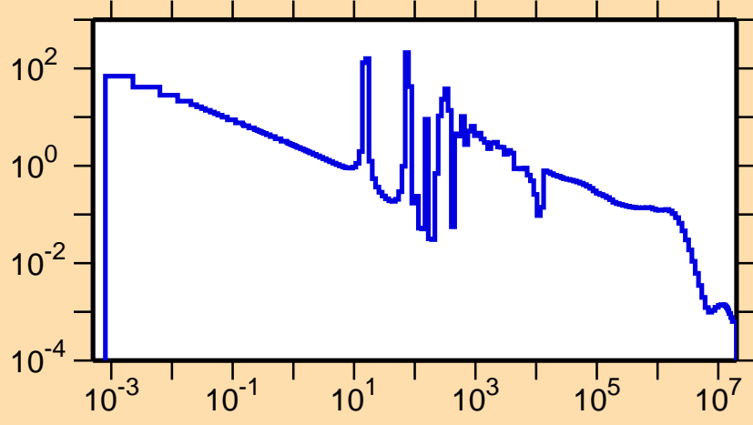
\sigma vs. E for ^{166}\text{Er}(n,\gamma)
