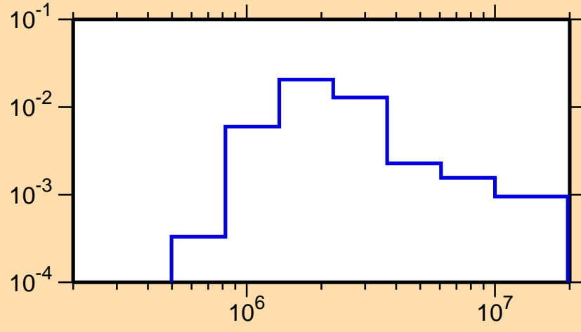
\sigma vs. E for ^{166}\text{Er}(n,n_3)
