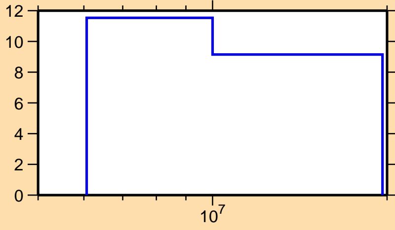
\Delta\sigma/\sigma vs. E for ^{166}\text{Er}(n,2n)
