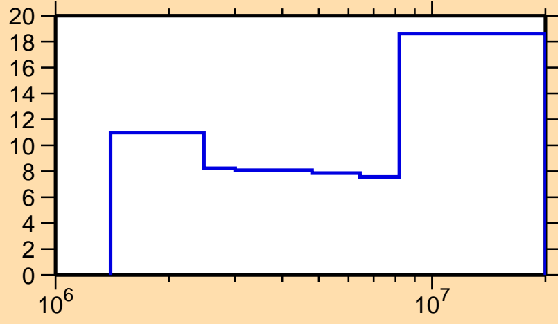
\Delta\sigma/\sigma vs. E for ^{166}\text{Er}(n,n\text{cont.})
