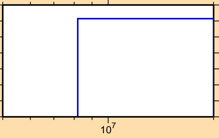
\sigma vs. E for ^{166}\text{Er}(n,t)
