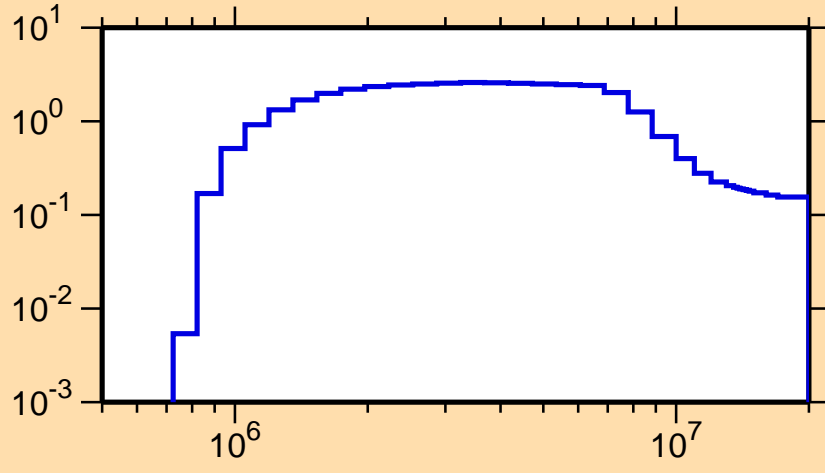
\sigma vs. E for ^{167}\text{Er}(n,n\text{cont.})
