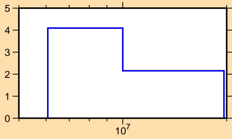
\Delta\sigma/\sigma vs. E for ^{167}\text{Er}(n,2n)
