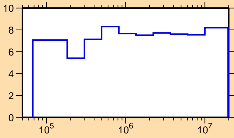
\Delta\sigma/\sigma vs. E for ^{167}\text{Er}(n,n_1)
