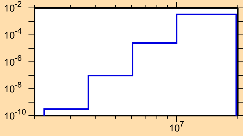
\sigma vs. E for ^{167}\text{Er}(n,p)
