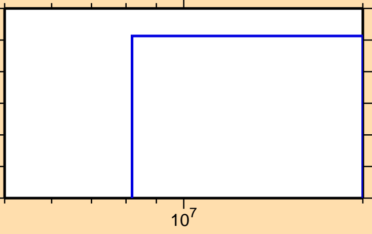
\sigma vs. E for ^{167}\text{Er}(n,p\alpha)
