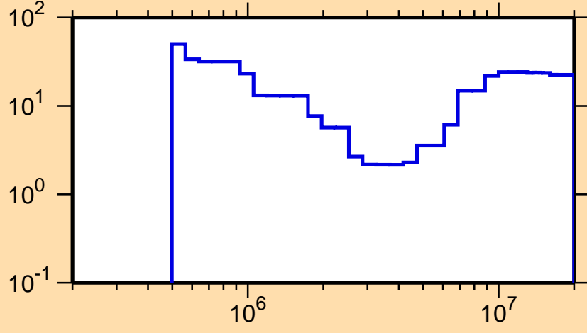
\Delta\sigma/\sigma vs. E for ^{167}\text{Er}(n,n\text{cont.})
