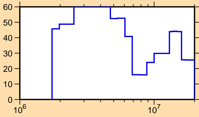
\Delta\sigma/\sigma vs. E for ^{167}\text{Er}(n,\gamma)
