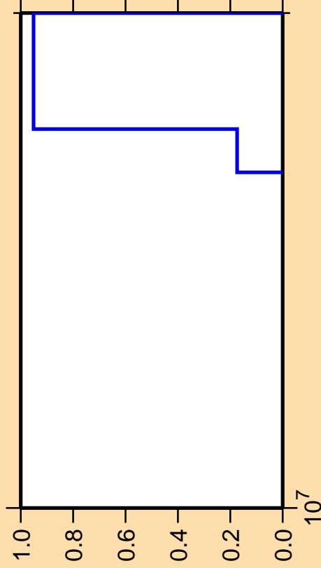
\Delta\sigma/\sigma vs. E for ^{167}\text{Er}(n,3n\alpha)
