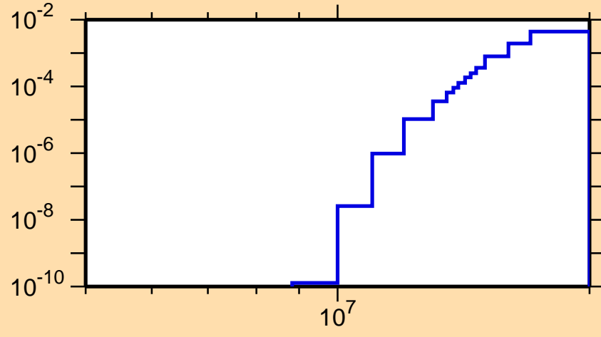
\sigma vs. E for ^{167}\text{Er}(n,np)
