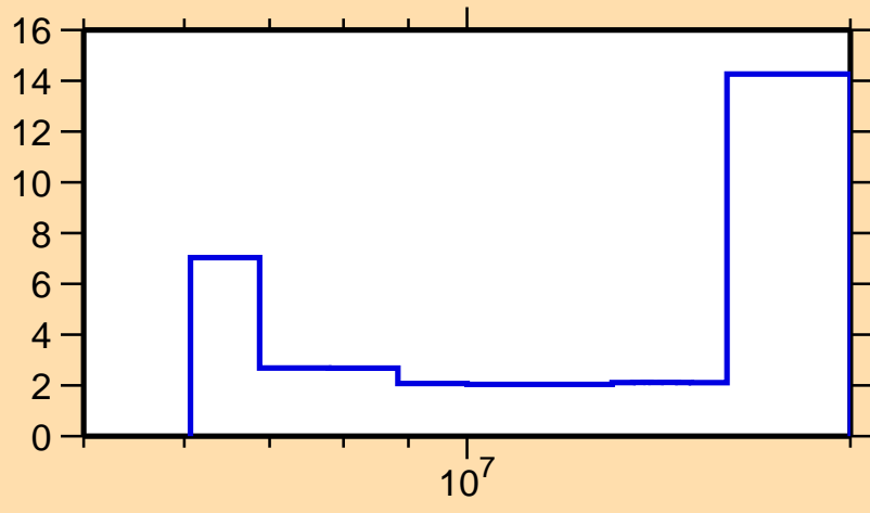
\Delta\sigma/\sigma vs. E for ^{167}\text{Er}(n,2n)
