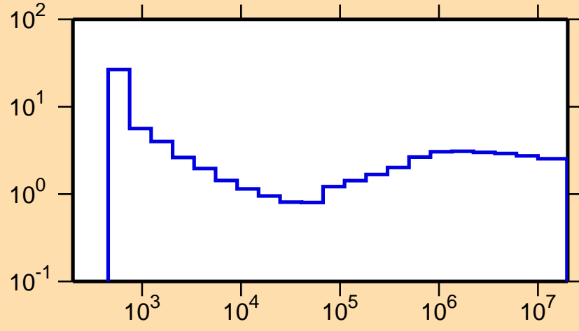
\sigma vs. E for ^{167}\text{Er}(n,\text{nonel.})
