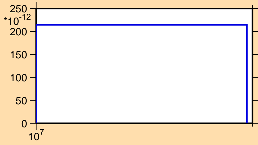
\sigma vs. E for ^{167}\text{Er}(n,nt)
