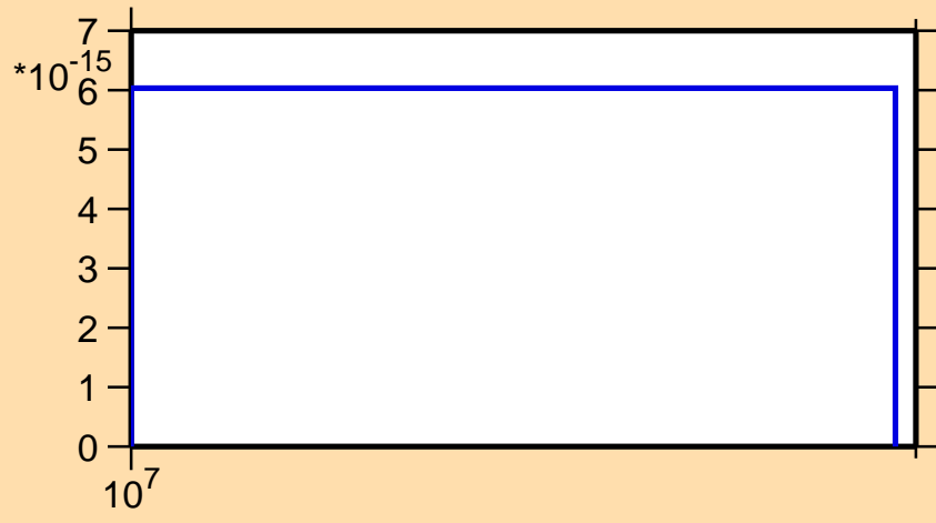
\sigma vs. E for ^{167}\text{Er}(n,3n\alpha)
