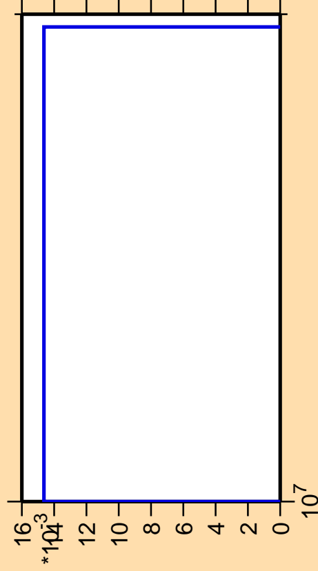
\Delta\sigma/\sigma vs. E for ^{167}\text{Er}(n,3n\alpha)
