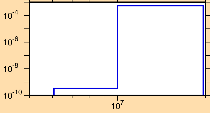
\sigma vs. E for ^{167}\text{Er}(n,d)
