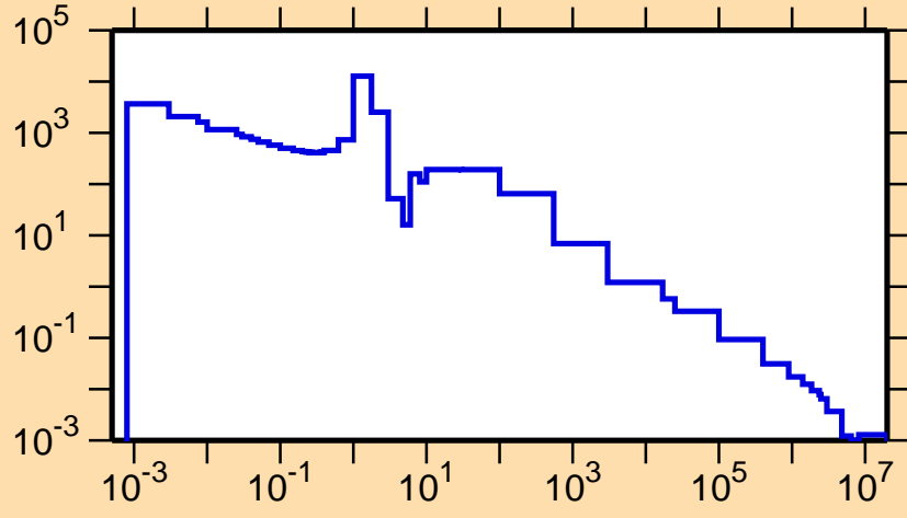
\sigma vs. E for ^{167}\text{Er}(n,\gamma)
