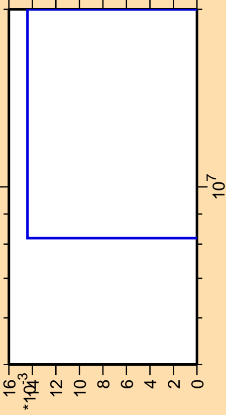
\Delta\sigma/\sigma vs. E for ^{167}\text{Er}(n,3n\alpha)
