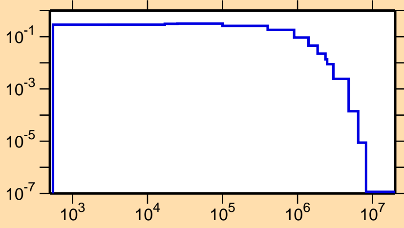
\sigma vs. E for ^{167}\text{Er}(n,n_1)
