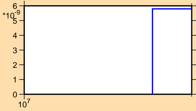
\sigma vs. E for ^{168}\text{Er}(n,2np)
