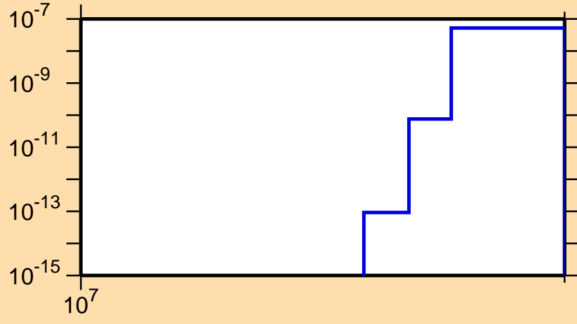
\sigma vs. E for ^{168}\text{Er}(n,\text{nd})
