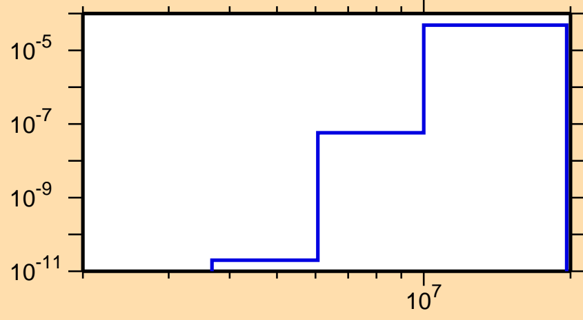
\sigma vs. E for ^{168}\text{Er}(n,n\alpha)
