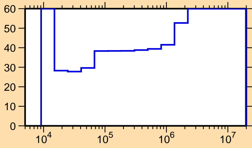
\Delta\sigma/\sigma vs. E for ^{168}\text{Er}(n,\gamma)
