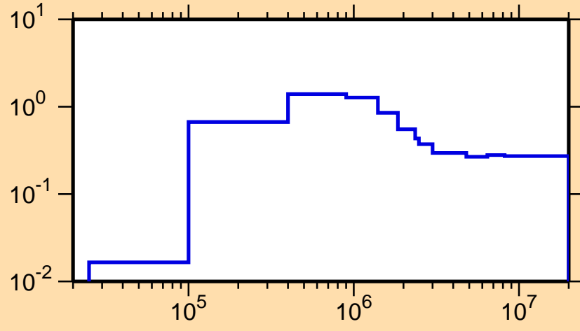
\sigma vs. E for ^{168}\text{Er}(n,n_1)
