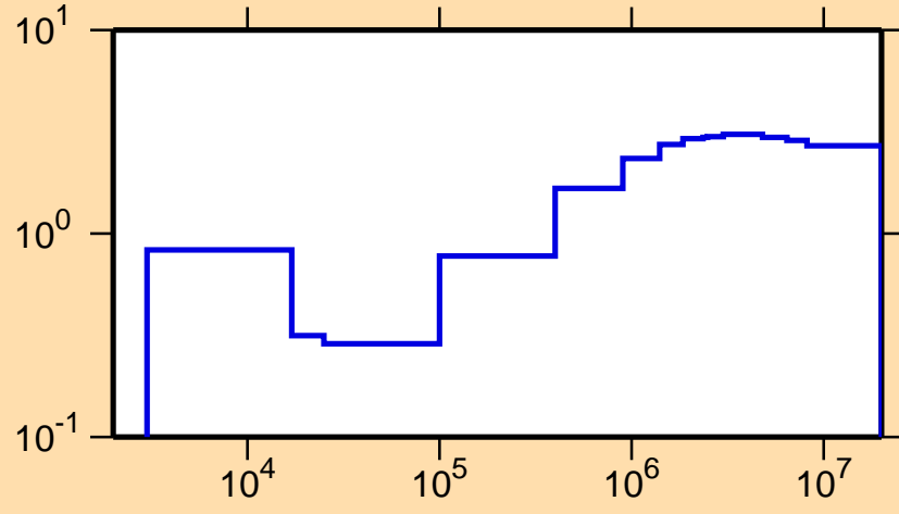
\sigma vs. E for ^{168}\text{Er}(n,\text{nonel.})
