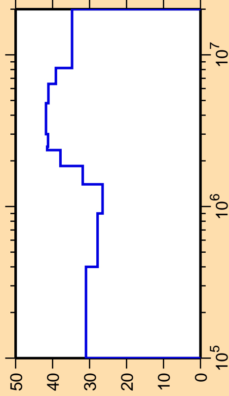
\Delta\sigma/\sigma vs. E for ^{168}\text{Er}(n,n_2)
