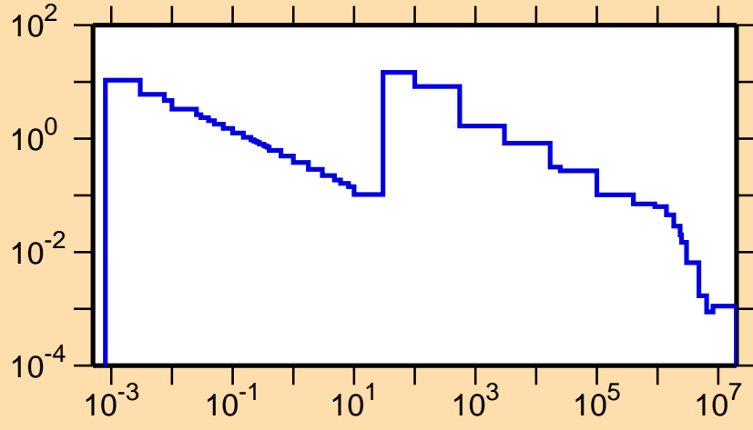
\sigma vs. E for ^{168}\text{Er}(n,\gamma)
