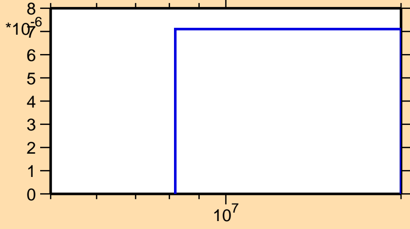
\sigma vs. E for ^{168}\text{Er}(n,t)
