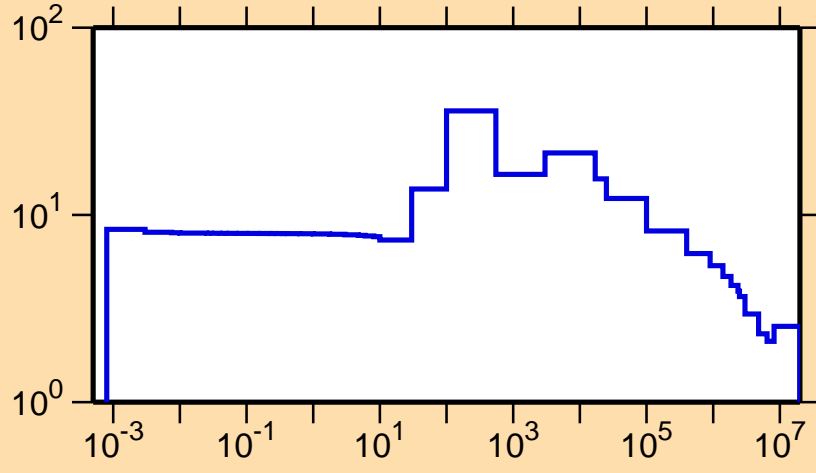
\sigma vs. E for ^{168}\text{Er}(n,\text{el.})
