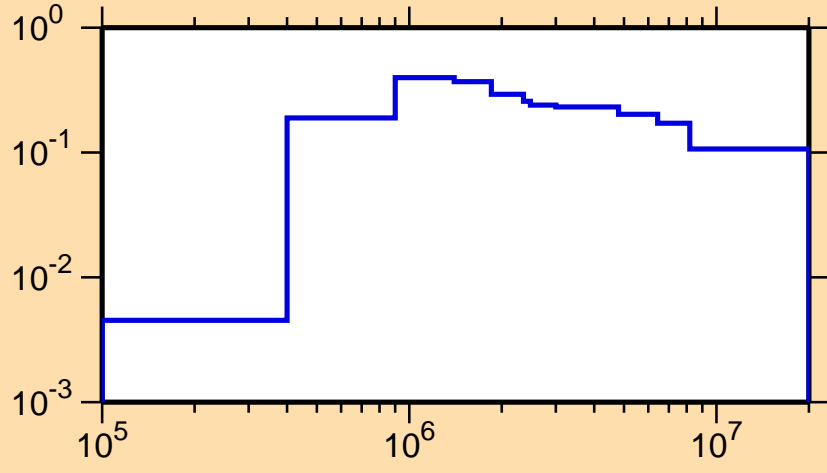
\sigma vs. E for ^{168}\text{Er}(n,n_2)
