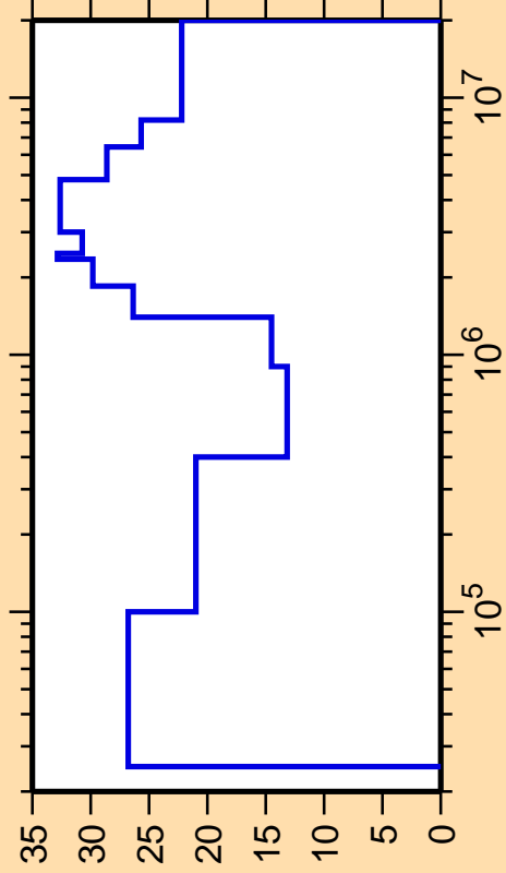
\Delta\sigma/\sigma vs. E for ^{168}\text{Er}(n,n_1)
