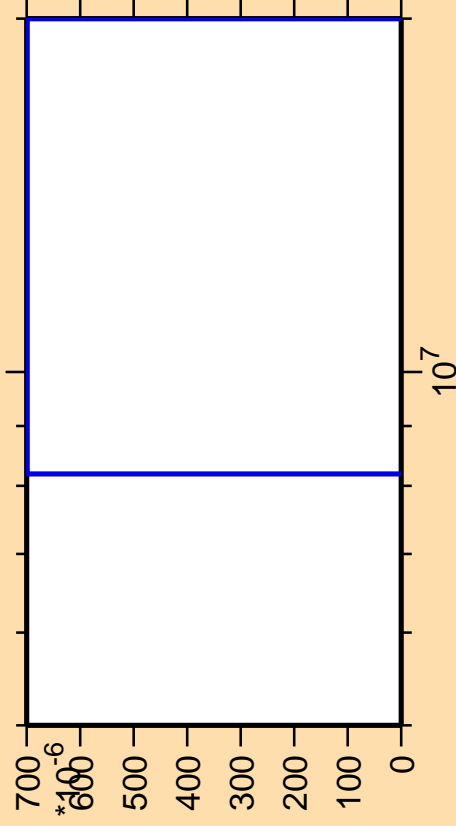
\Delta\sigma/\sigma vs. E for ^{168}\text{Er}(n,3n\alpha)
