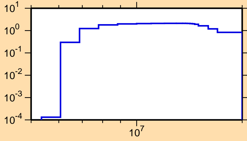
\sigma vs. E for ^{169}\text{Er}(n,2n)
