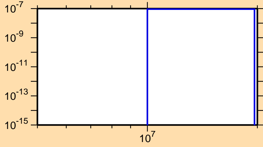
\sigma vs. E for ^{169}\text{Er}(n,2n\alpha)
