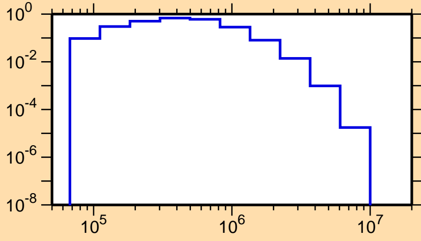
\sigma vs. E for ^{169}\text{Er}(n,n_2)
