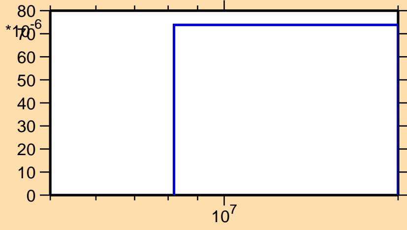
\sigma vs. E for ^{169}\text{Er}(n,np)
