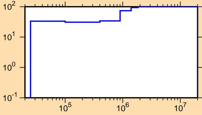
\Delta\sigma/\sigma vs. E for ^{169}\text{Er}(n,n_1)
