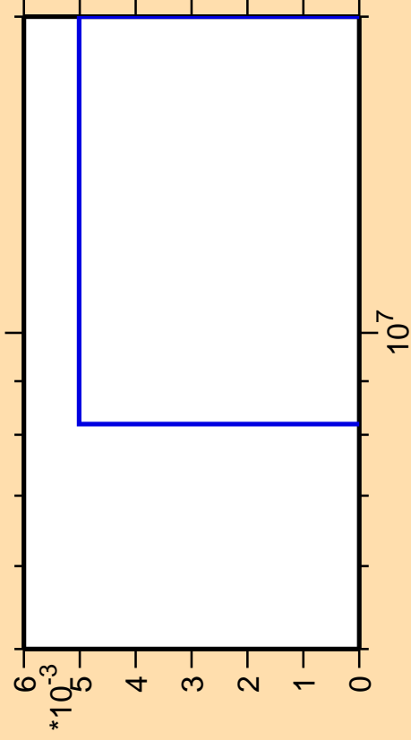
\Delta\sigma/\sigma vs. E for ^{169}\text{Er}(n,3n\alpha)
