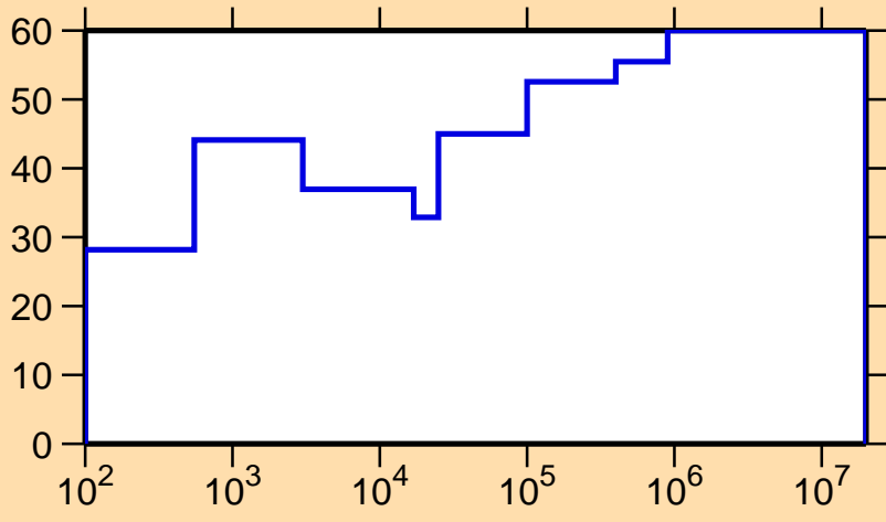
\Delta\sigma/\sigma vs. E for ^{169}\text{Er}(n,\gamma)
