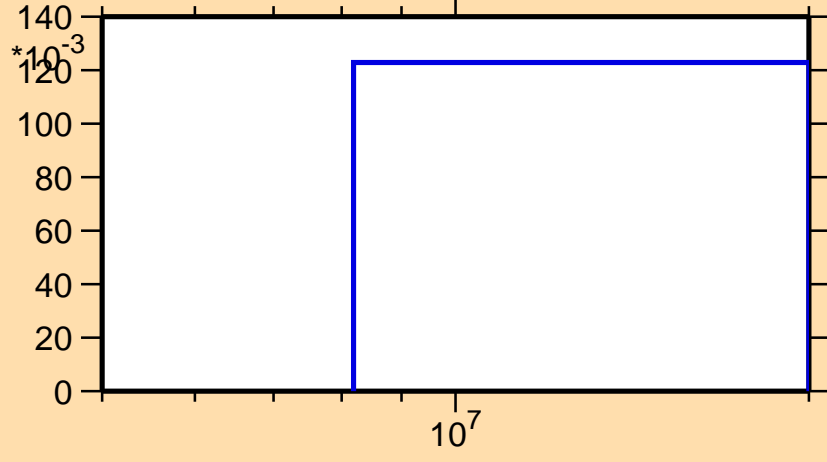
\sigma vs. E for ^{169}\text{Er}(n,3n)
