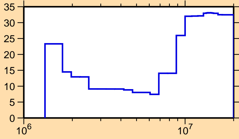
\Delta\sigma/\sigma vs. E for ^{170}\text{Er}(n,n\text{cont.})
