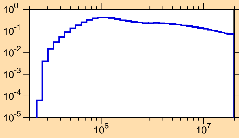
\sigma vs. E for ^{170}\text{Er}(n,n_2)
