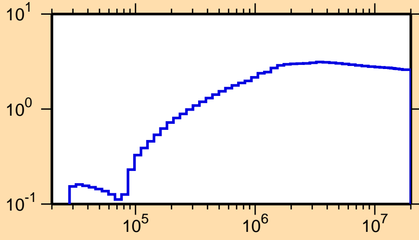
\sigma vs. E for ^{170}\text{Er}(n,\text{nonel.})
