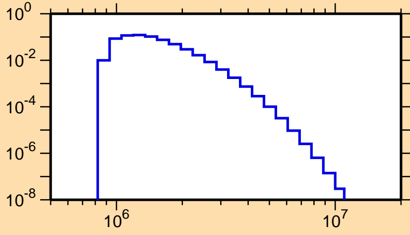
\sigma vs. E for ^{170}\text{Er}(n,n_4)
