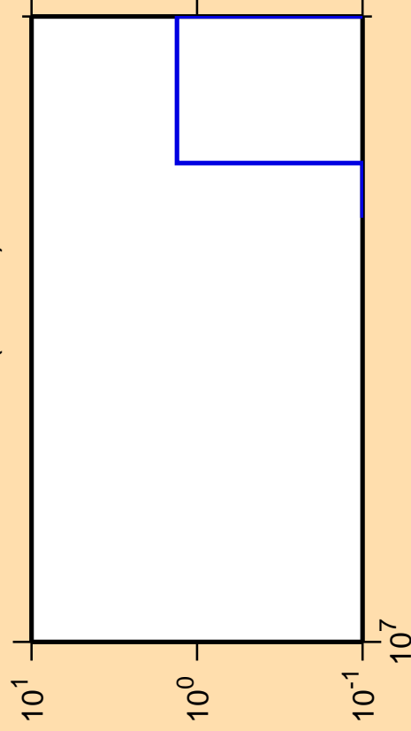
\Delta\sigma/\sigma vs. E for ^{170}\text{Er}(n,3n\alpha)
