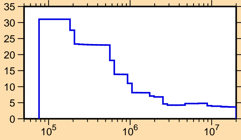
\Delta\sigma/\sigma vs. E for ^{170}\text{Er}(n,\text{nonel.})
