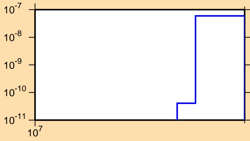
\sigma vs. E for ^{170}\text{Er}(n,nt)
