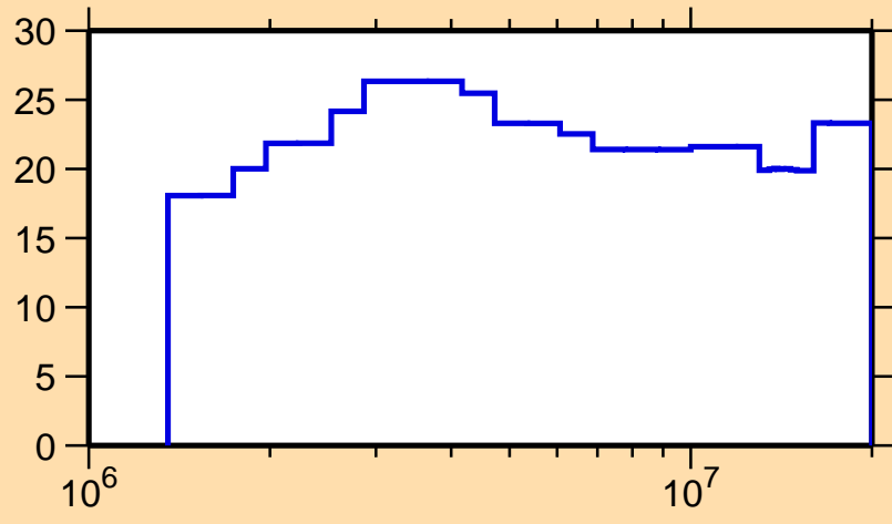
\Delta\sigma/\sigma vs. E for ^{170}\text{Er}(n,n_1)
