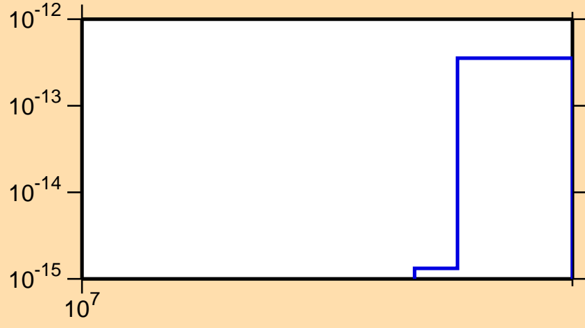
\sigma vs. E for ^{170}\text{Er}(n,3n\alpha)
