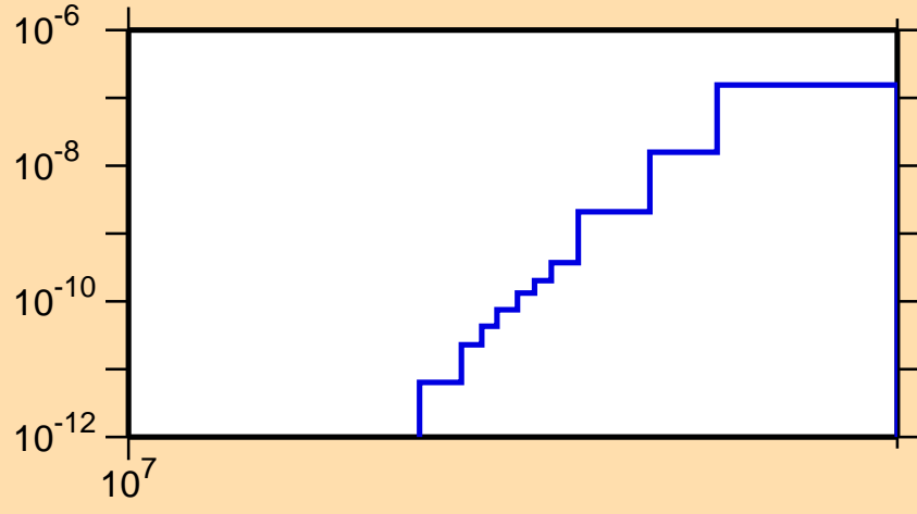
\sigma vs. E for ^{170}\text{Er}(n,2n\alpha)
