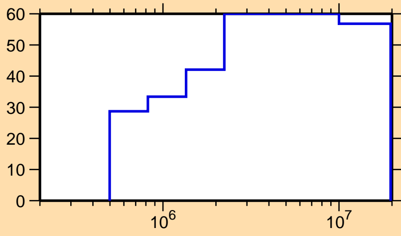
\Delta\sigma/\sigma vs. E for ^{170}\text{Er}(n,\gamma)
