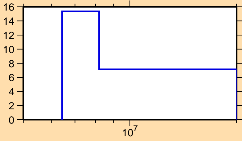
\Delta\sigma/\sigma vs. E for ^{170}\text{Er}(n,2n)
