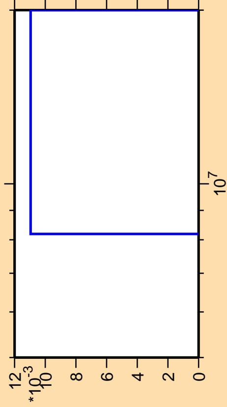
\Delta\sigma/\sigma vs. E for ^{170}\text{Er}(n,3n\alpha)
