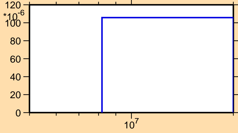
\sigma vs. E for ^{170}\text{Er}(n,d)
