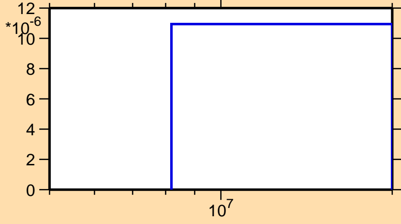
\sigma vs. E for ^{170}\text{Er}(n,t)
