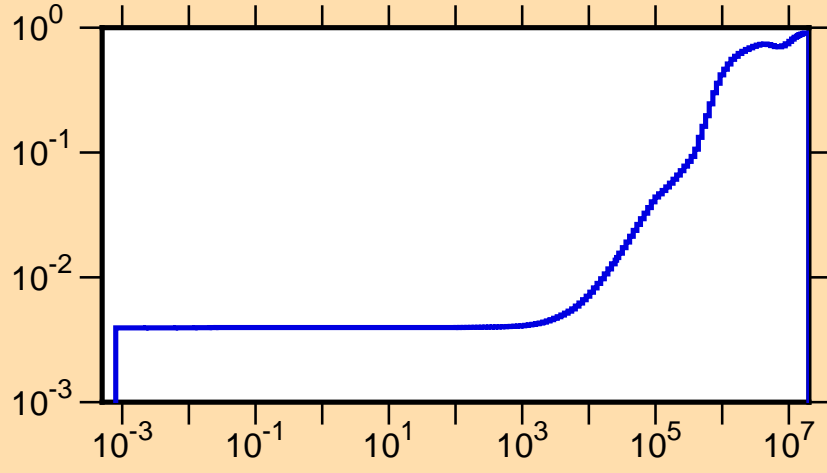
\mu vs. E for ^{171}\text{Er}(\text{mt251})
