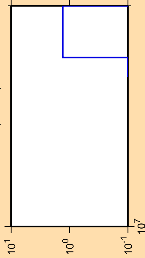
\Delta\sigma/\sigma vs. E for ^{171}\text{Er}(n,3n\alpha)
