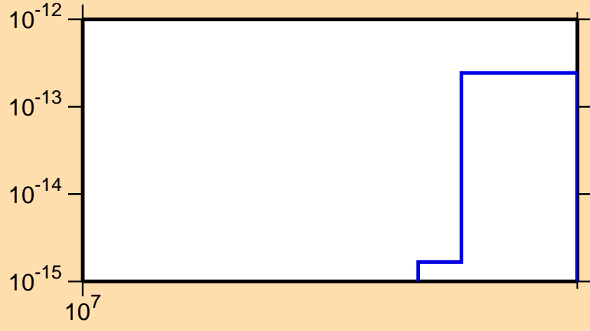
\sigma vs. E for ^{171}\text{Er}(n,3n\alpha)
