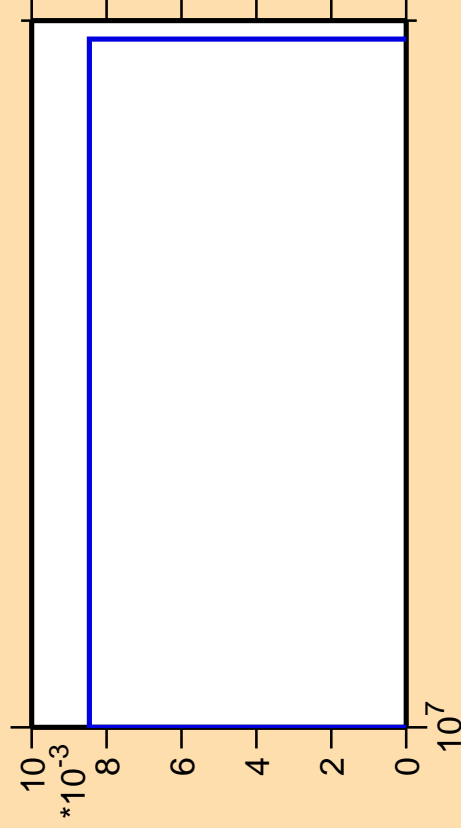
\Delta\sigma/\sigma vs. E for ^{171}\text{Er}(n,3n\alpha)
