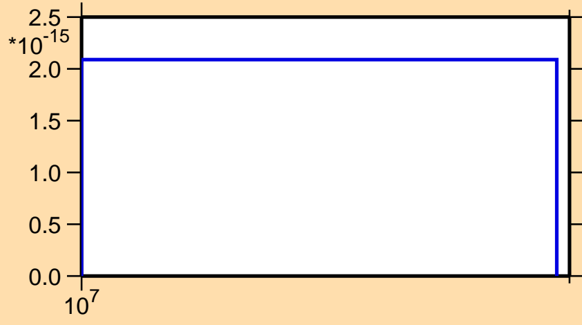
\sigma vs. E for ^{171}\text{Er}(n,3n\alpha)
