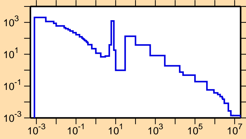
\sigma vs. E for ^{171}\text{Er}(n,\gamma)
