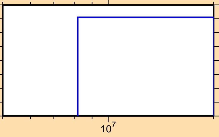
\sigma vs. E for ^{171}\text{Er}(n,t)
