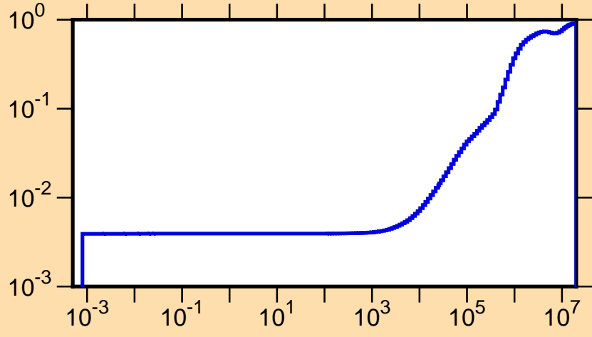
\mu vs. E for ^{172}\text{Er}(\text{mt251})
