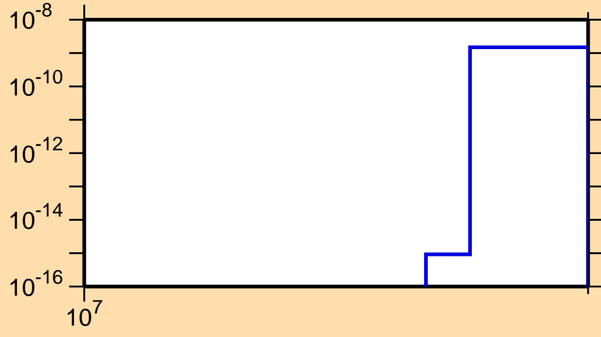
\sigma vs. E for ^{172}\text{Er}(n,2np)
