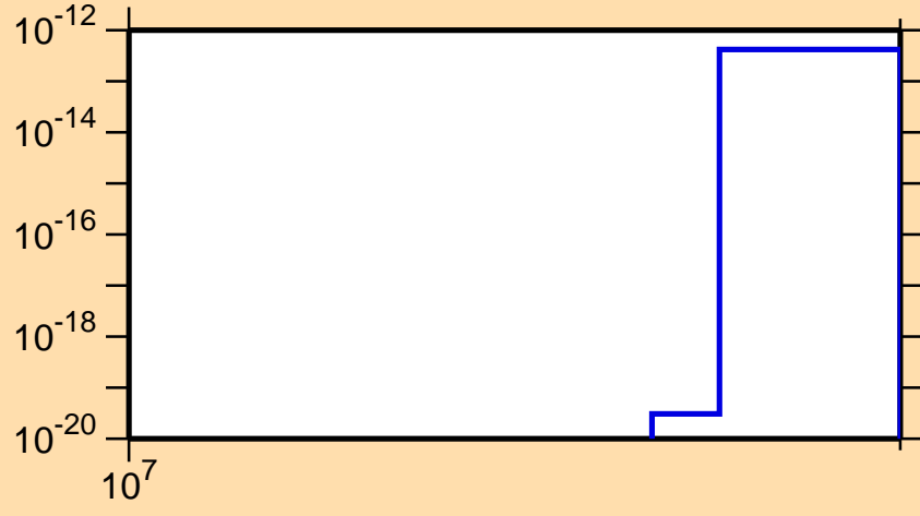
\sigma vs. E for ^{172}\text{Er}(n,3n\alpha)
