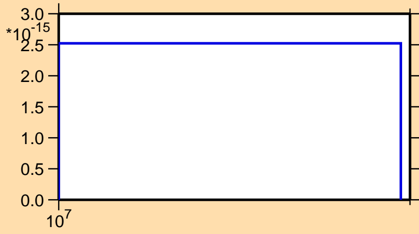
\sigma vs. E for ^{172}\text{Er}(n,3n\alpha)
