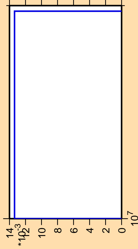
\Delta\sigma/\sigma vs. E for ^{172}\text{Er}(n,3n\alpha)
