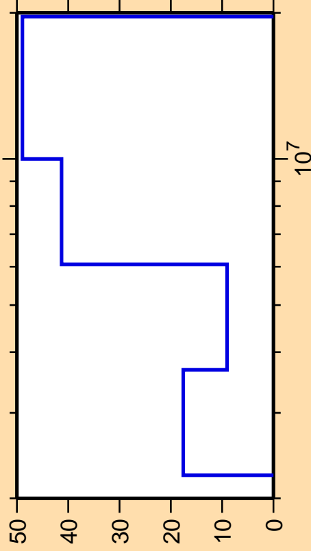
\Delta\sigma/\sigma vs. E for ^{172}\text{Er}(n,n\text{cont.})
