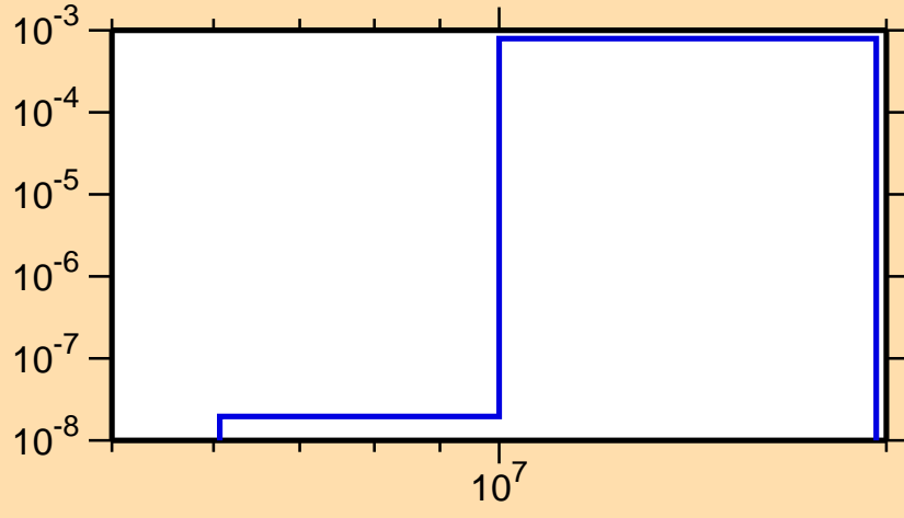
\sigma vs. E for ^{172}\text{Er}(n,p)
