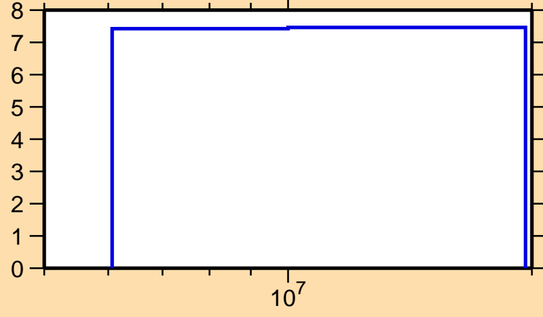
\Delta\sigma/\sigma vs. E for ^{172}\text{Er}(n,\text{el.})
