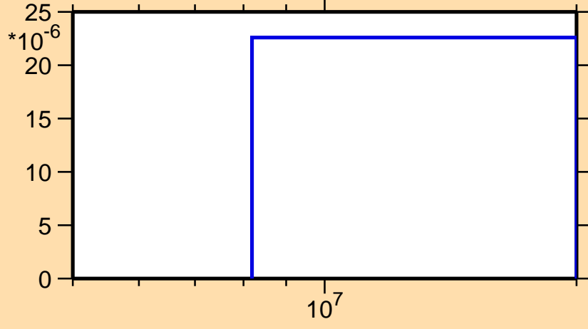
\sigma vs. E for ^{172}\text{Er}(n,d)
