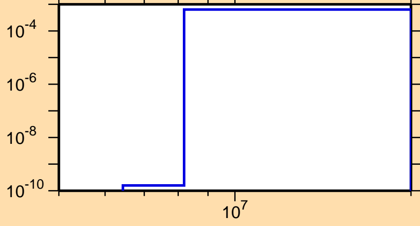
\sigma vs. E for ^{172}\text{Er}(n,p)
