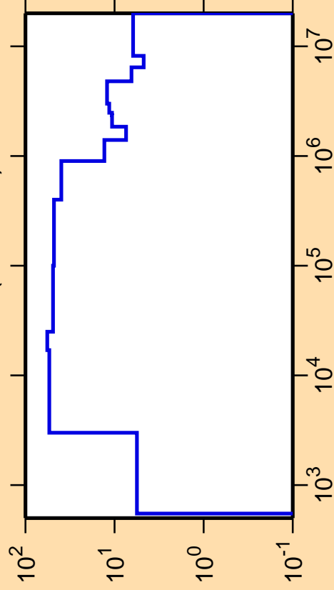
\Delta\sigma/\sigma vs. E for ^{172}\text{Er}(n,\text{nonel.})
