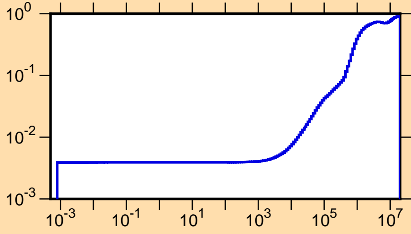
\mu vs. E for ^{173}\text{Er}(\text{mt251})
