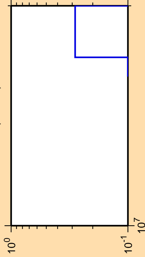
\Delta\sigma/\sigma vs. E for ^{173}\text{Er}(n,3n\alpha)
