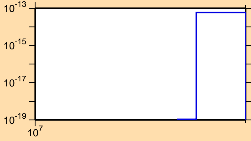
\sigma vs. E for ^{173}\text{Er}(n,3n\alpha)
