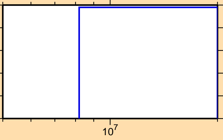
\sigma vs. E for ^{173}\text{Er}(n,d)
