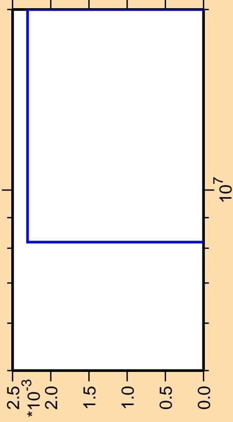
\Delta\sigma/\sigma vs. E for ^{173}\text{Er}(n,3n\alpha)
