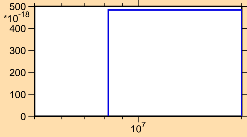
\sigma vs. E for ^{173}\text{Er}(n,3n\alpha)
