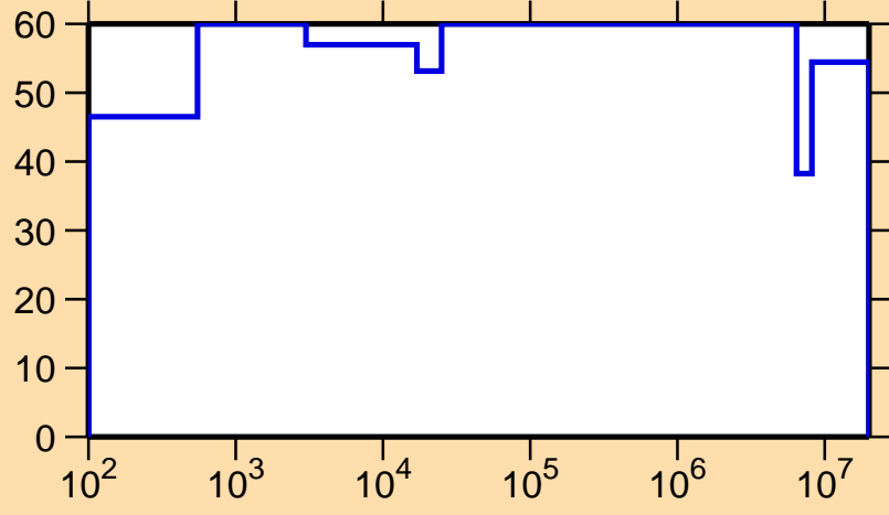
\Delta\sigma/\sigma vs. E for ^{173}\text{Er}(n,\gamma)
