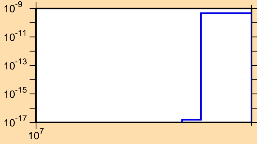
\sigma vs. E for ^{174}\text{Er}(n,2np)
