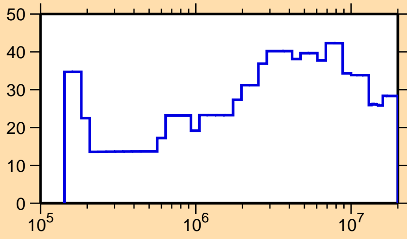
\Delta\sigma/\sigma vs. E for ^{174}\text{Er}(n, el.)
