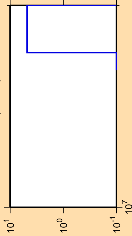
\Delta\sigma/\sigma vs. E for ^{174}\text{Er}(n,3n\alpha)
