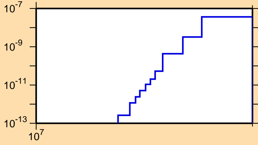
\sigma vs. E for ^{174}\text{Er}(n,2n\alpha)
