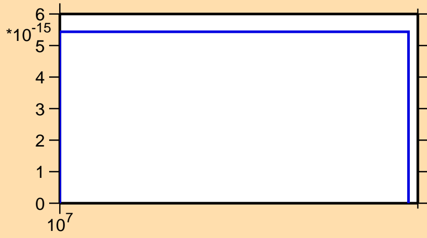
\sigma vs. E for ^{174}\text{Er}(n,3n\alpha)
