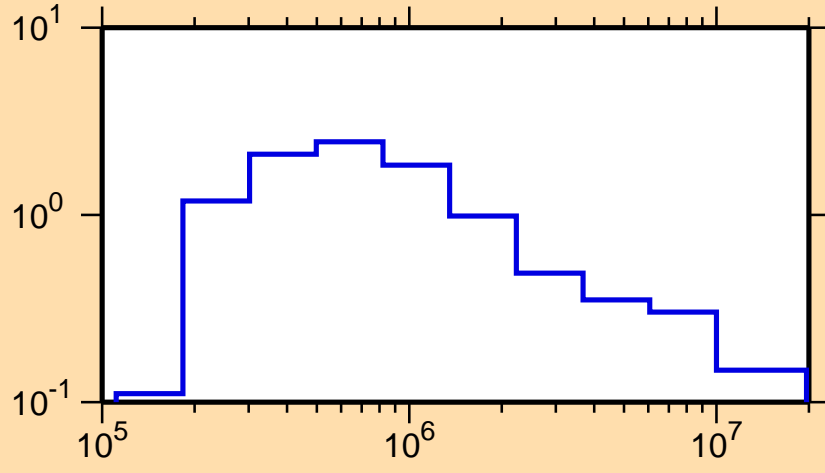
\sigma vs. E for ^{174}\text{Er}(n,n_1)
