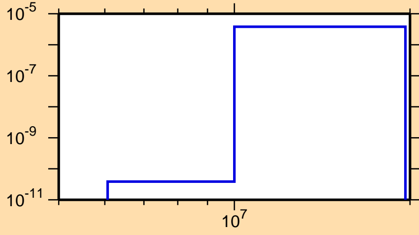
\sigma vs. E for ^{174}\text{Er}(n,n\alpha)
