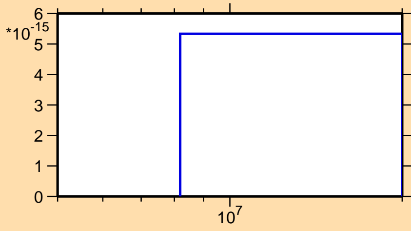
\sigma vs. E for ^{174}\text{Er}(n,3n\alpha)
