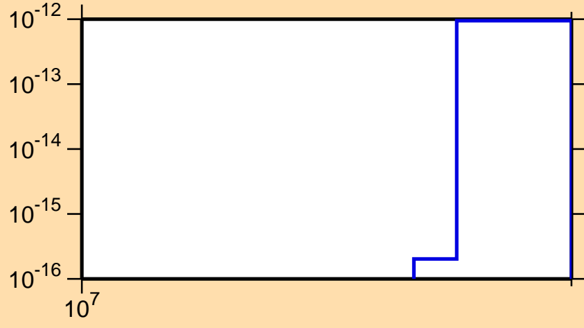
\sigma vs. E for ^{175}\text{Er}(n,3n\alpha)
