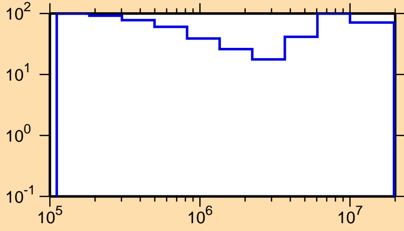
\Delta\sigma/\sigma vs. E for ^{175}\text{Er}(n,n\text{cont.})
