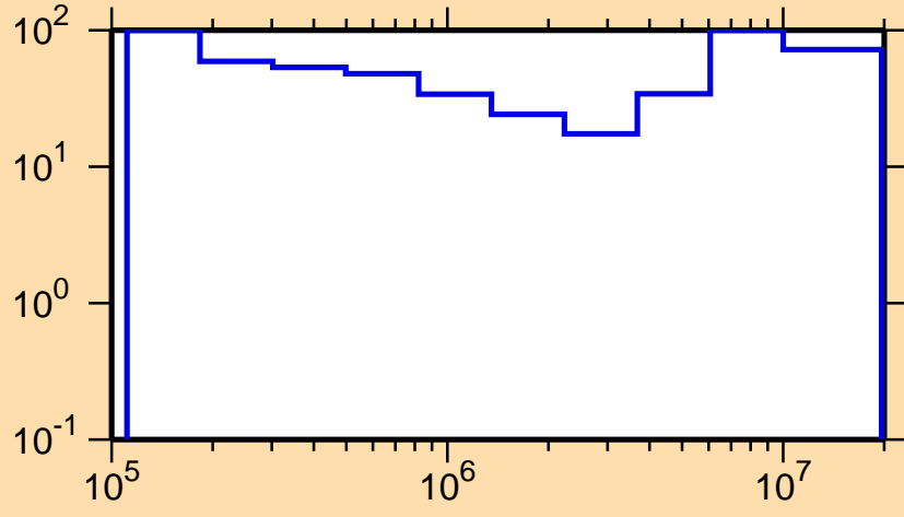
\Delta\sigma/\sigma vs. E for ^{175}\text{Er}(n, \text{inel.})
