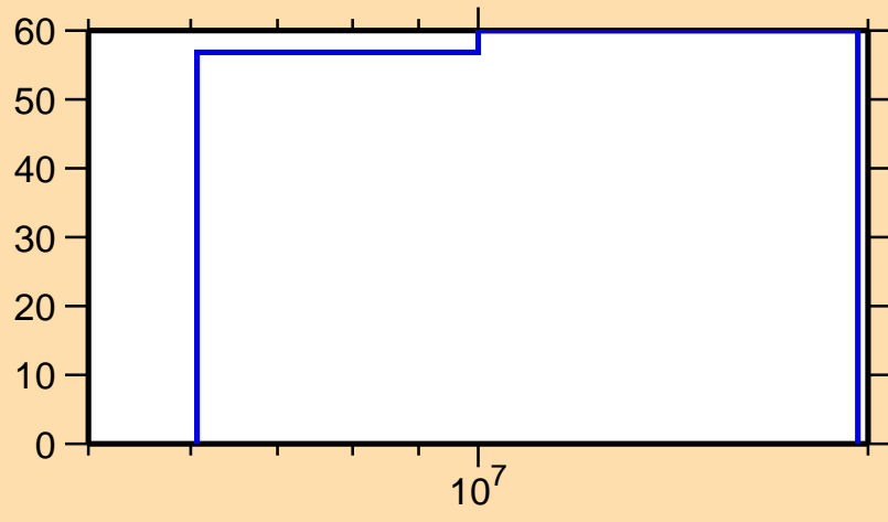
\Delta\sigma/\sigma vs. E for ^{175}\text{Er}(n,\gamma)
