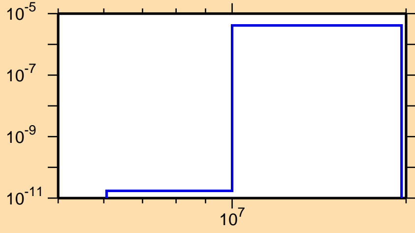
\sigma vs. E for ^{175}\text{Er}(n,n\alpha)
