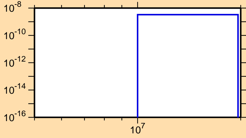
\sigma vs. E for ^{175}\text{Er}(n,2n\alpha)
