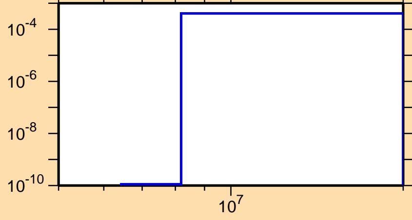
\sigma vs. E for ^{175}\text{Er}(n,p)
