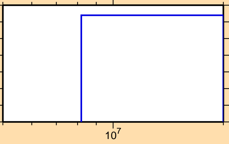
\sigma vs. E for ^{175}\text{Er}(n,d)
