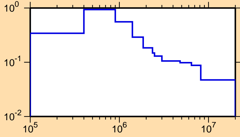
\sigma vs. E for ^{175}\text{Er}(n,n_1)
