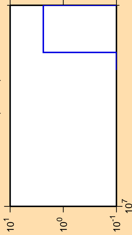
\Delta\sigma/\sigma vs. E for ^{176}\text{Er}(n,3n\alpha)
