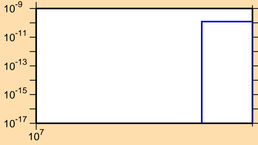
\sigma vs. E for ^{176}\text{Er}(n,2np)
