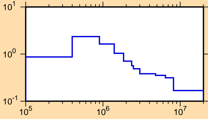
\sigma vs. E for ^{176}\text{Er}(n,n_1)
