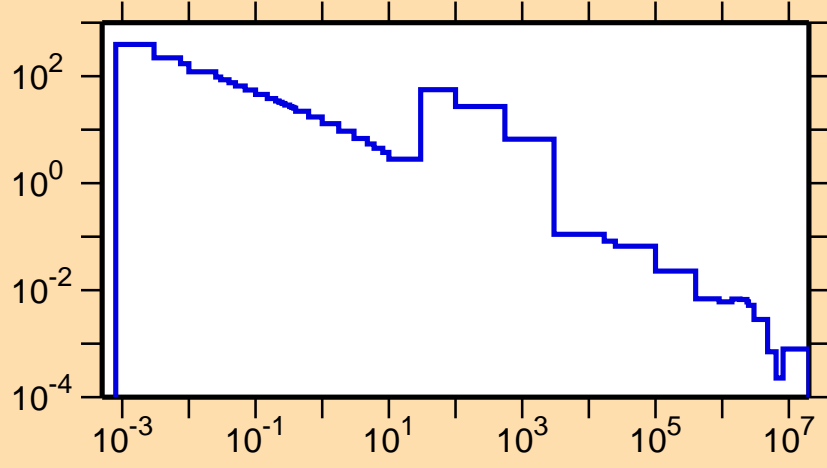
\sigma vs. E for ^{176}\text{Er}(n,\gamma)
