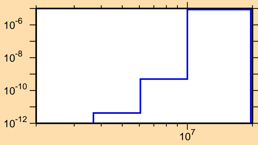
\sigma vs. E for ^{177}\text{Er}(n,\alpha)
