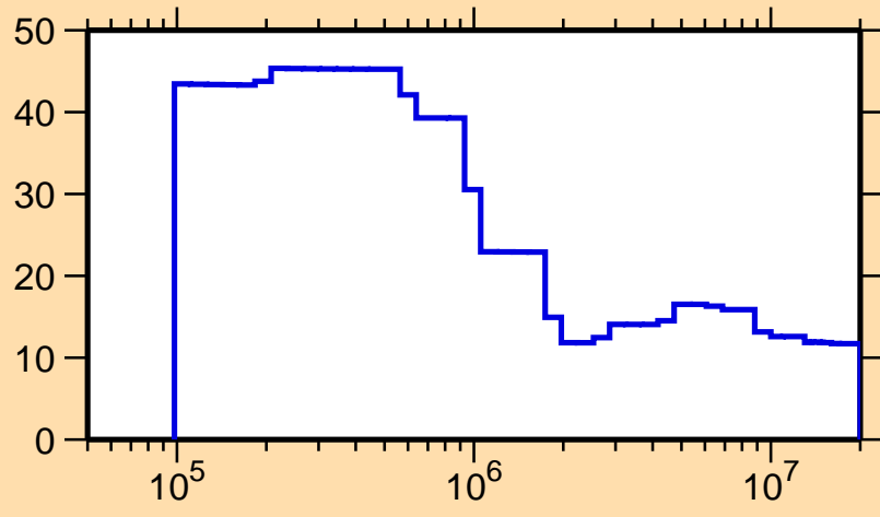
\Delta\sigma/\sigma vs. E for ^{239}\text{Es}(n,\text{tot.})
