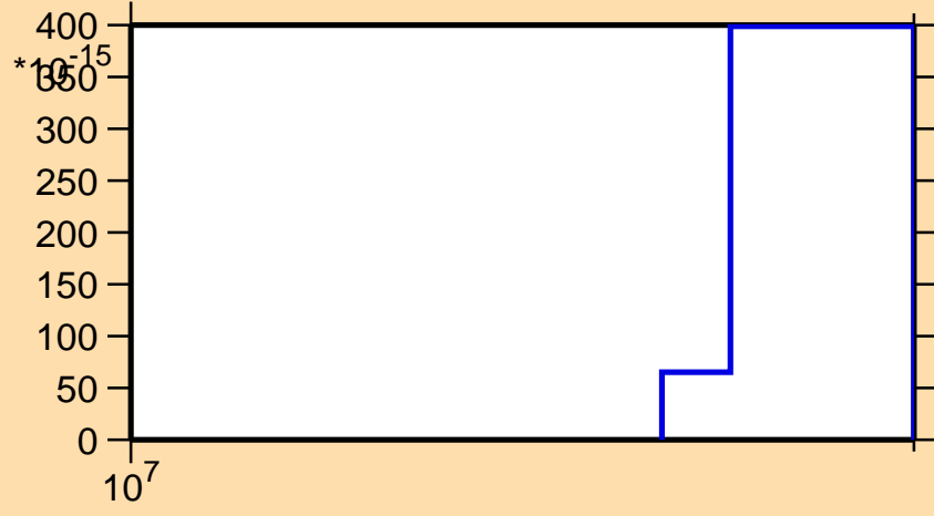
\sigma vs. E for ^{239}\text{Es}(n,pd)
