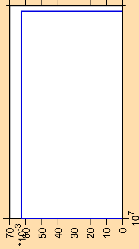
\Delta\sigma/\sigma vs. E for ^{239}\text{Es}(n,pd)
