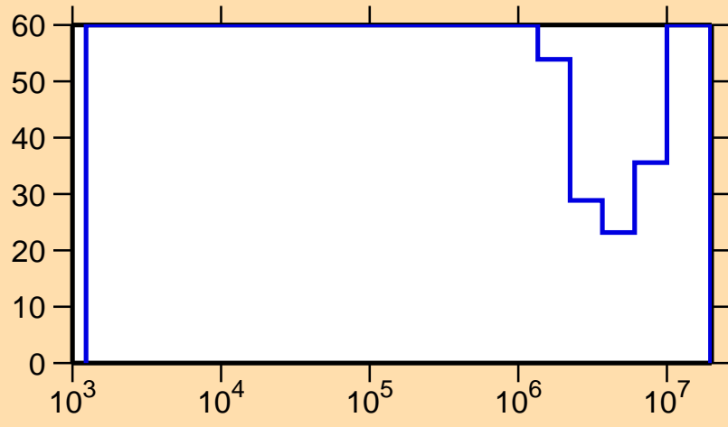
\Delta\sigma/\sigma vs. E for ^{239}\text{Es}(n,p)
