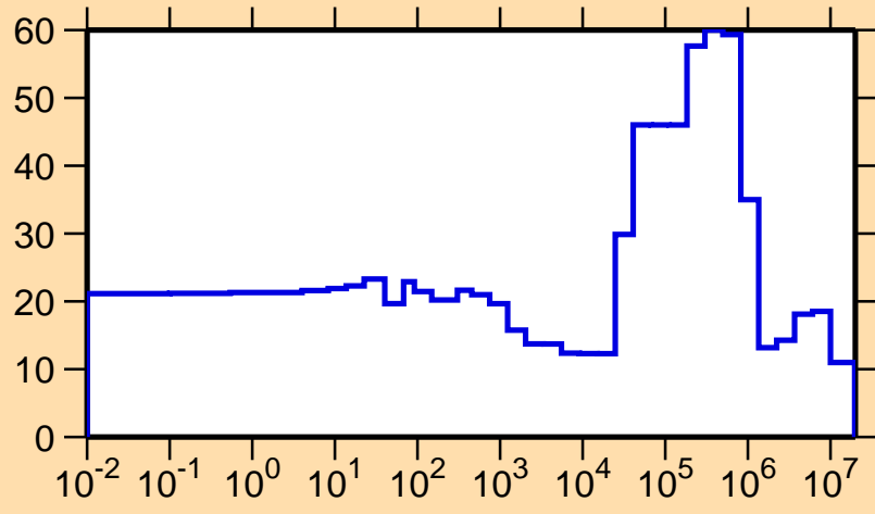
\Delta\sigma/\sigma vs. E for ^{239}\text{Es}(n,el.)
