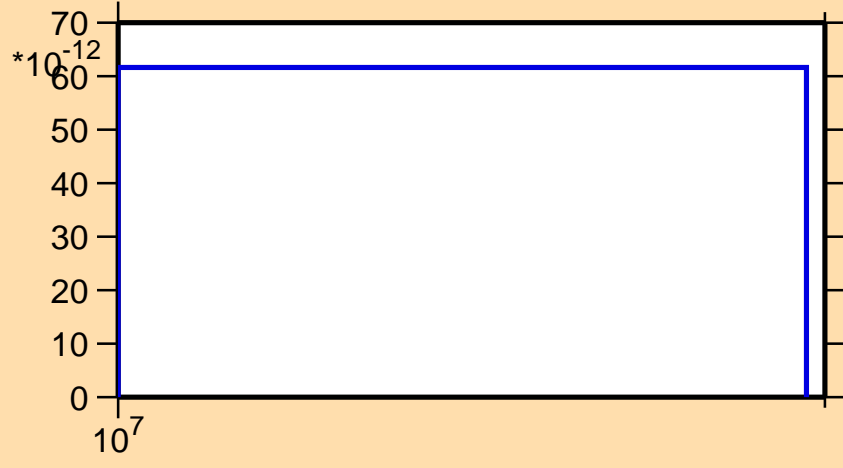
\sigma vs. E for ^{239}\text{Es}(n,nd)
