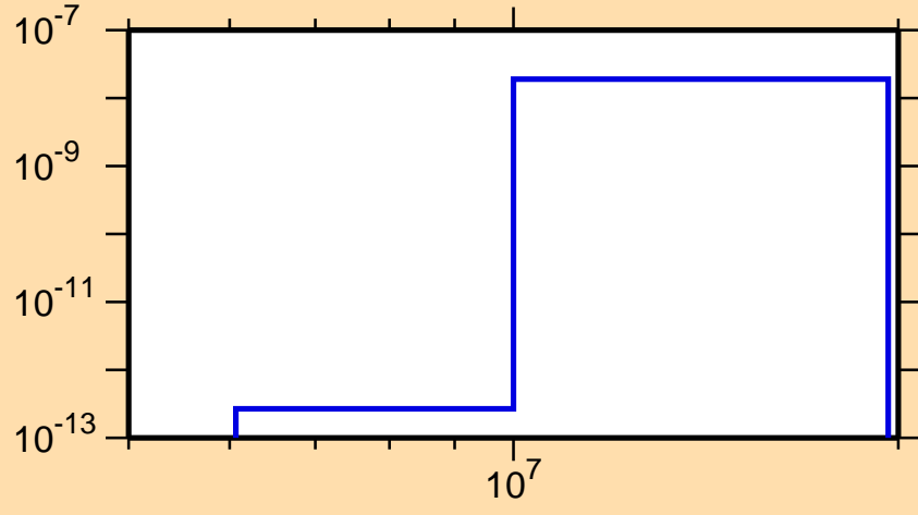
\sigma vs. E for ^{239}\text{Es}(n,\text{He3})
